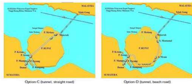
Figure 3a. Corridor I: Dumai-Rupat island-Malaysia, with 4 Options: Bridge for Option A dan B, Tunnel for Option C and D (continuation)
